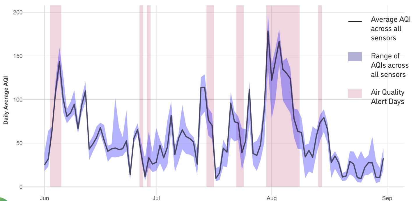
Figure 3: Average AQI across All Sensors for Days with AQAs
